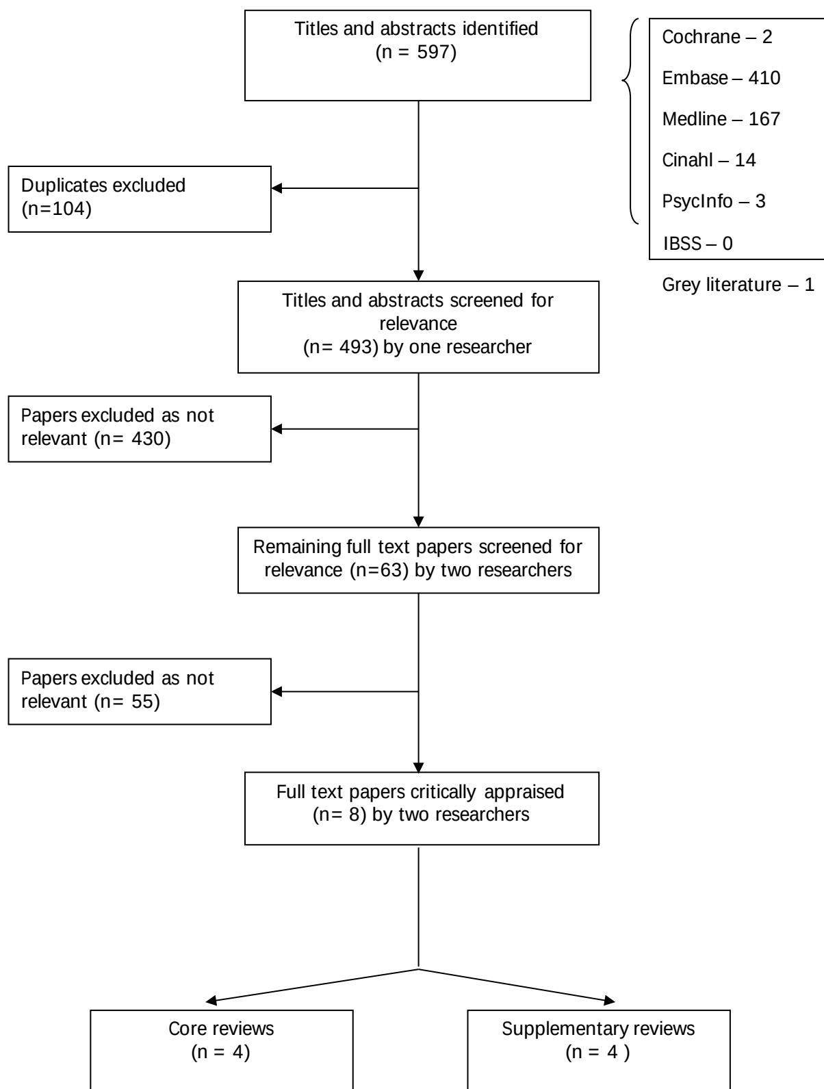
Figure B. Flow chart of reviews retrieved in the update of the RoR (covering the period March 2007– March 2011)
